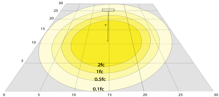
6W 3000K, Area 30'x 30' Mounting Height: 9'
